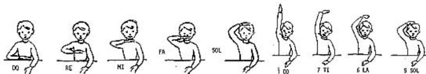
Diagram 2: melodic gestures
